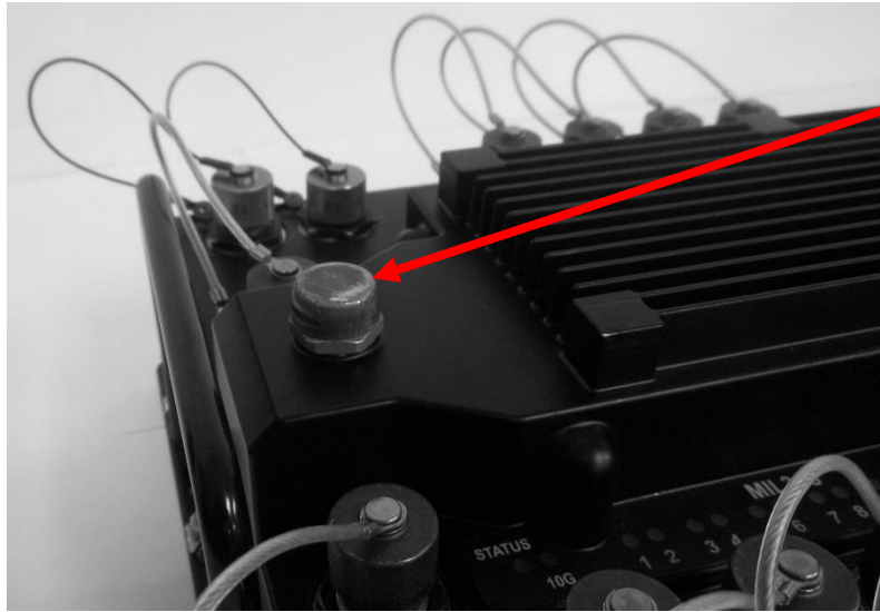
Pressure Vent
